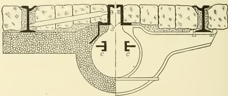
Fig. 241. Conduit for Underground Trolley System
